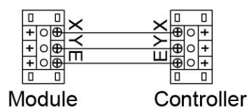
Incorrect connection
