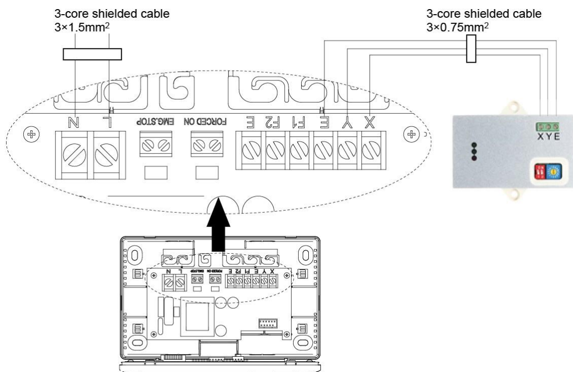
Incorrect connection
